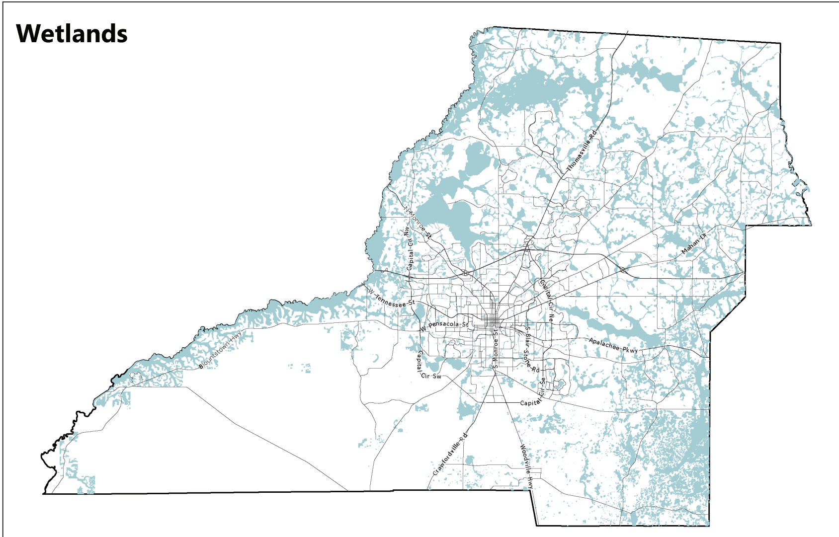
Map 13: Wetlands
