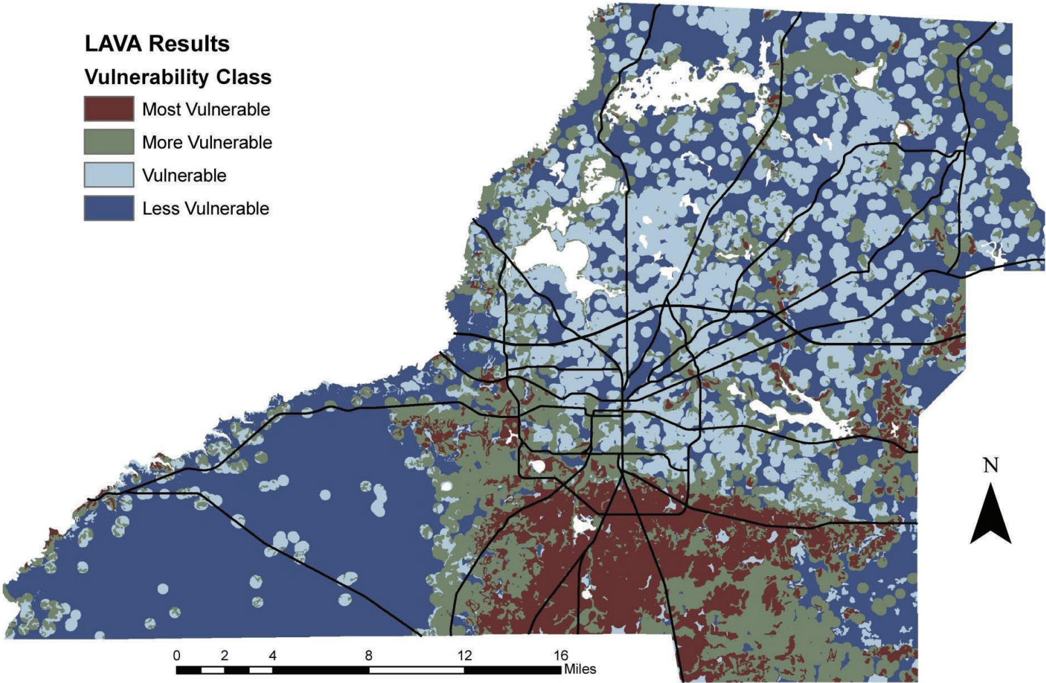
Map 18: LAVA Results
